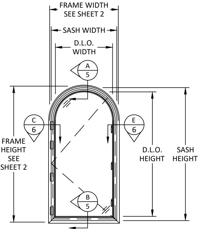
TYPICAL ELEVATION SINGLE CASEMENT, ROUND TOP
