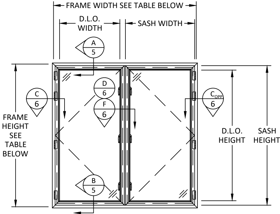
TYPICAL ELEVATION FRENCH CASEMENT
