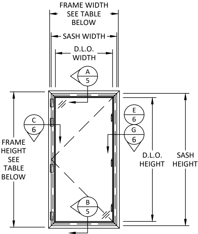
TYPICAL ELEVATION SINGLE CASEMENT
