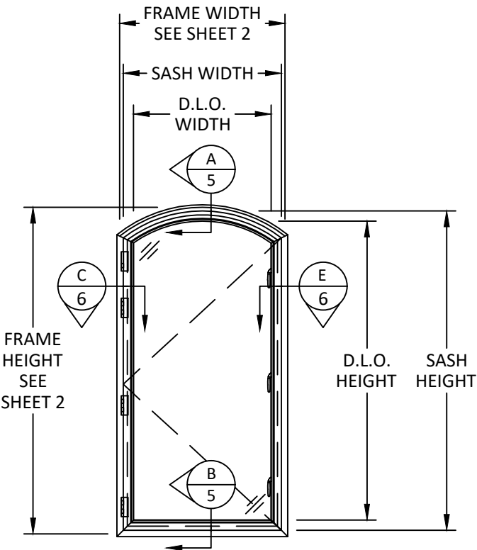
TYPICAL ELEVATION SINGLE CASEMENT, ARCH TOP
